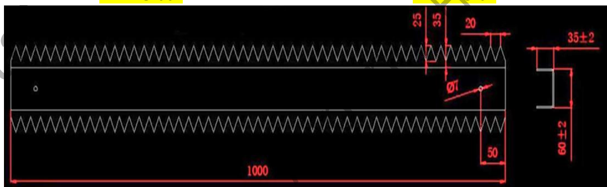
HWWS-06 Drawing
