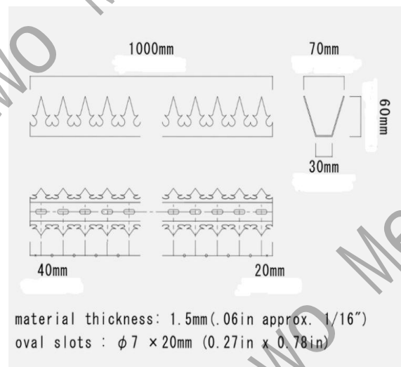
Type 4. Customized wall spikes: HWWS-04: 1.5mm thick material, with 1000mm length
