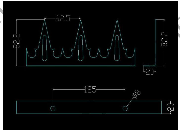
Type 6. Customized wall spikes: HWWS-06: 2.0mm thick material, with 1000mm length
