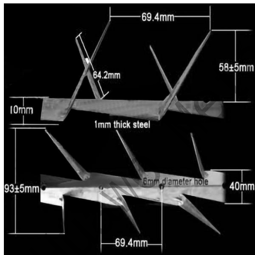
Type 3. Small size wall spikes(HWWS-03): 1250mm long, with 1.0mm thick material.
